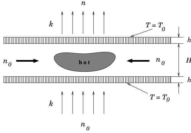
Figure 2: Combustion in a continuous flow reactor.
