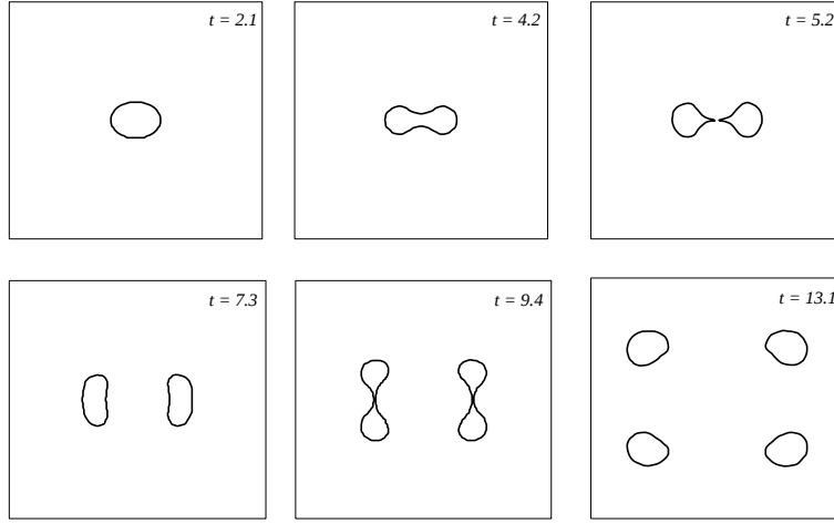
Figure 4: Self-replication of a spot. Result of the numerical solution of Eq. (5.4). The box is 50 \times 50 . Other parameters are: \Lambda = 4 , \delta = 18.3 , based on the model in Eq. (1.7) and (1.8) with \epsilon = 10^{-4} , A - A_b^- = 0.0455 .
