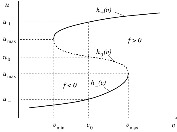
Figure 3: The activator nullcline (closeup).
