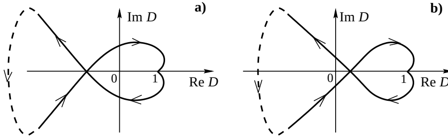
FIG. B.1. A qualitative form of the function D(\omega) for large values of C (a) and for small values of C (b).
