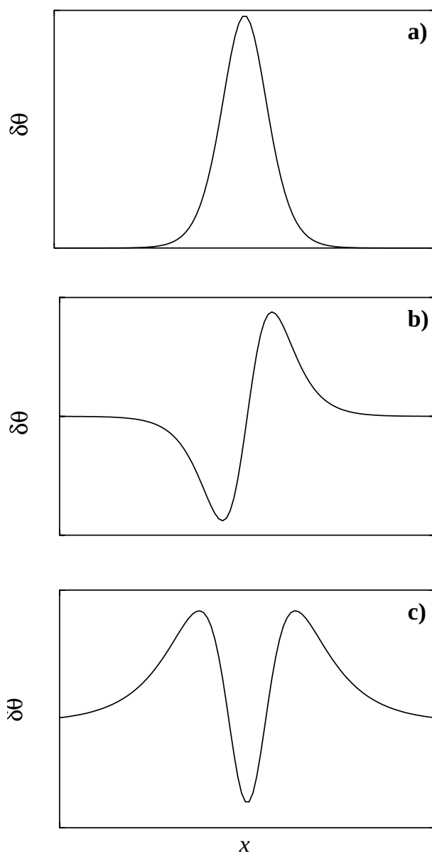
FIG. 2.1. A qualitative form of the lowest-lying modes \delta\theta_n .
