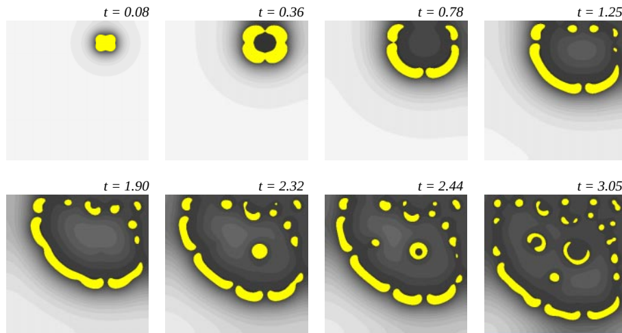
Fig. 5. Splitting as a result of the formation and the breakdown of a quasi one-dimensional wave. Results of the numerical solution of equations (11) and (12) with \epsilon = 0.05 , \alpha = 0.1 , and A = 3 . The system is 5 \times 5 . The shades of gray show the distribution of \eta . The spots show the regions where \theta > 10 .
