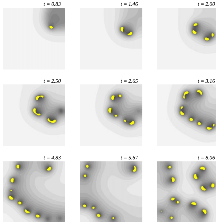
Fig. 7. Formation of spatio-temporal chaos. Results of the numerical solution of equations (11) and (12) with \epsilon = 0.1 , \alpha = 0.04 , and A = 1 . The system is 10 \times 10 . The shades of gray show the distribution of \eta . The spots show the regions where \theta > 5 .
