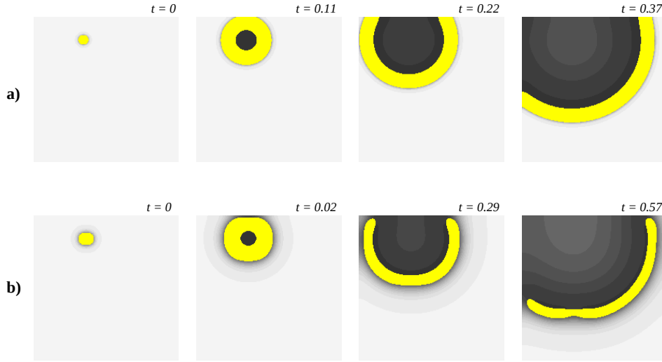
Fig. 8. Propagation of waves in the Gray-Scott model. Results of the numerical solution of equations (11) and (12) with (a) \epsilon = 0.2 , \alpha = 0.05 , and A = 1.5 ; (b) \epsilon = 0.1 , \alpha = 0.05 , A = 1.5 . In (a) the system is 10 \times 10 ; in (b) the system is 5 \times 5 . The shades of gray show the distribution of \eta . The spots show the regions where \theta > 0 .
