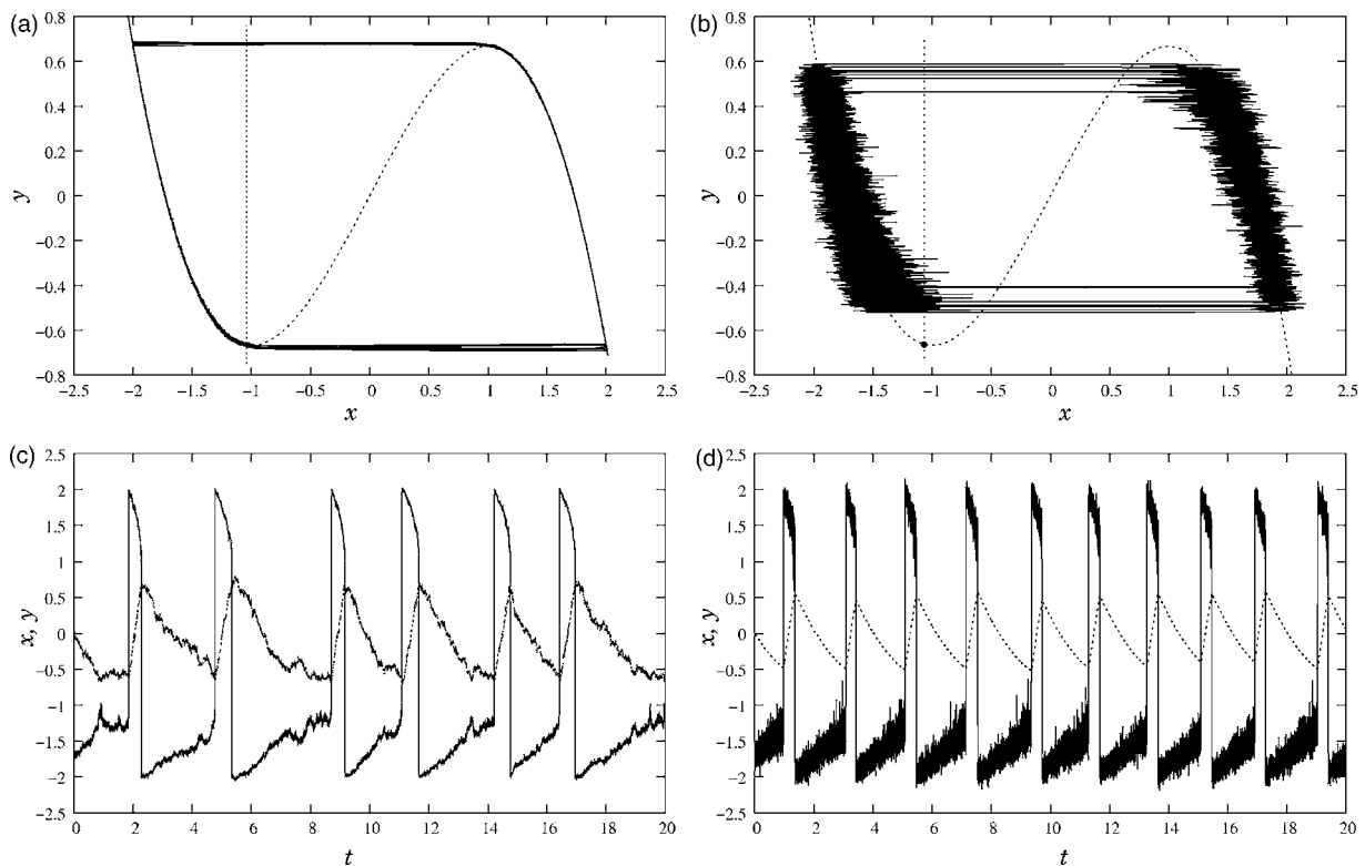
FIG. 2. Two types of limit cycle behaviors observed in the numerical simulations of (1a) and (1b) with a=1.05 . (a) and (c): \varepsilon=10^{-4} , \delta_1=0 , \delta_2=0.2 (CR); (b) and (d): \varepsilon=10^{-4} , \delta_1=0.2 , \delta_2=0 (SISR). In (a) and (b), the phase portrait is shown, whereas in (c) and (d), the time traces of both x and y are shown. In 2(a) and 2(b), the dotted lines indicate the nullclines.
