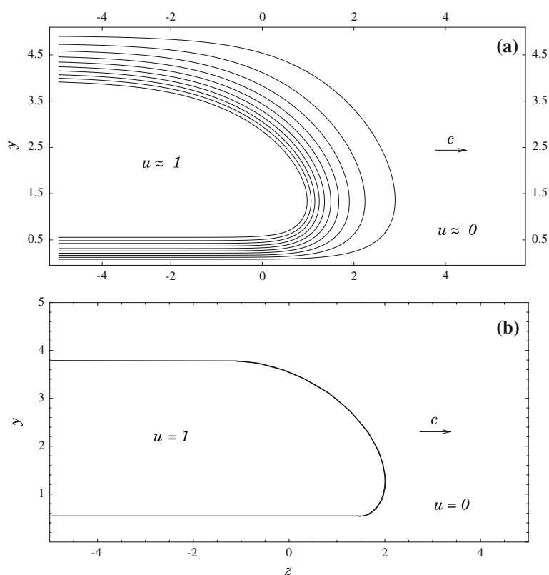
Fig. 4 Comparison of the front profiles for \varphi = y and L = \frac{5}{2} . a The level curves of the numerical solution of (1.4) and (6.12) with \varepsilon = 0.2 . b The curve minimizing \Pi_c with c = c^\sharp
