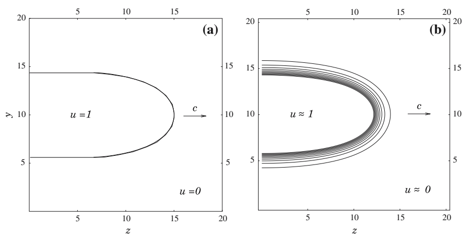
Fig. 5 Comparison of the front profiles for \varphi_y = -2 \cos\left(\frac{\pi y}{2L}\right) and L = 10 . a The minimizer of \Pi_c for c = c^\sharp . b The level curves of the numerical solution of (1.4) and (6.12) with \varepsilon = 0.2
