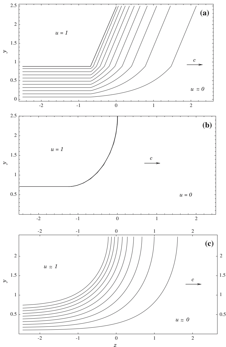
Fig. 2 Comparison of the front profiles obtained from different approximations in the case \varphi = 0 and L = \frac{5}{2} . a The level curves of the trial function u_{\lambda, \mu, l} for c = 0.925 and the parameters \lambda, \mu, l obtained from minimizing \Phi_c^0[u_{\lambda, \mu, l}] . b The curve minimizing \Pi_C with c = c^\sharp . c The level curves of the numerical solution of (1.4) and (6.12) for \varepsilon = 0.2 . Only the lower half of u is shown in all cases
