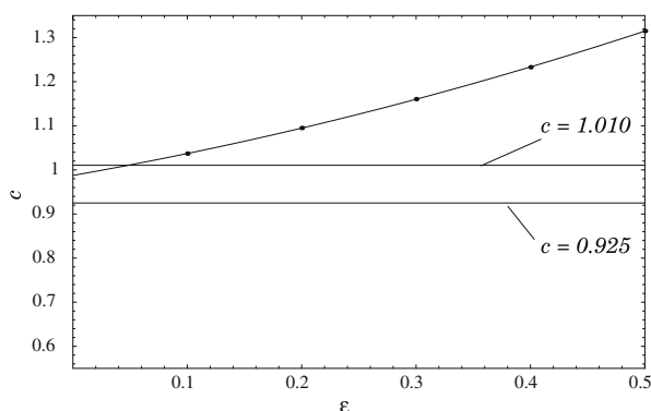
Fig. 3 Dependence of c_\epsilon^+ obtained from the numerical solution of (1.4) and (6.12) with \varphi = 0 . The dots are the results of the simulations, the curve is a fit using a quadratic polynomial c_\epsilon^+ \simeq 0.987 + 0.458\epsilon + 0.393\epsilon^2 . Numerical solutions of (1.4) and the propagation speeds are obtained by solving the associated parabolic problem in (1.1) on a rectangle (0, 5) \times (0, 20) with the initial data u(y, z) = \cosh^{-2}(\frac{1}{2}\sqrt{(y - \frac{5}{2})^2 + z^2}) discretized on the 100 \times 400 grid (except for \epsilon = 0.1 when a 200 \times 800 grid was used), with Dirichlet boundary conditions everywhere except at z = 0 , where Neumann boundary conditions are used
