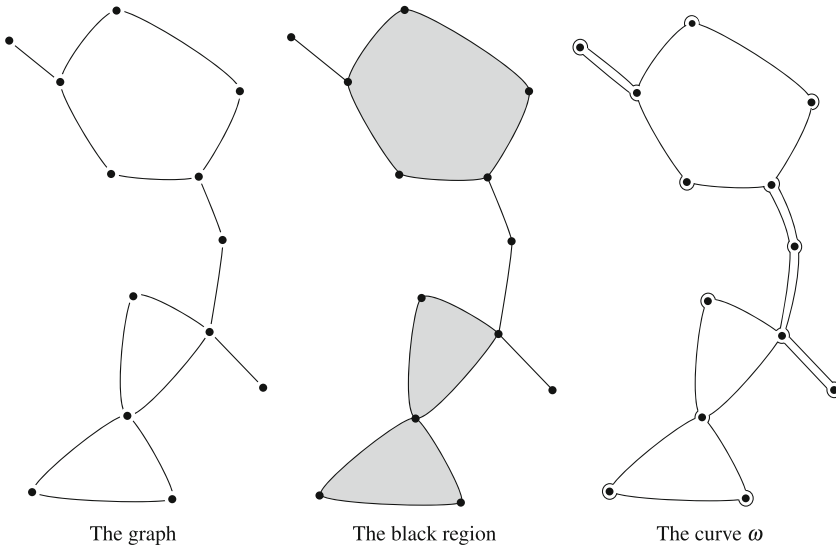
Fig. 1 Desingularization of a graph
