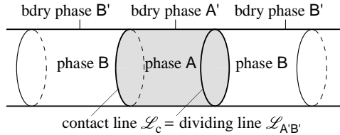
Fig. 9. Equilibrium configuration for v_2 \leq v .
