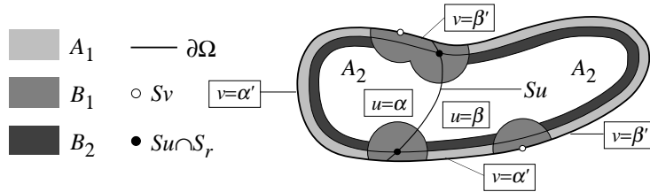
Fig. 6. The partition of \Omega .
