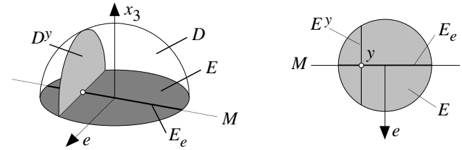
Fig. 4. The sets D , E , E_e , E^y and D^y .
